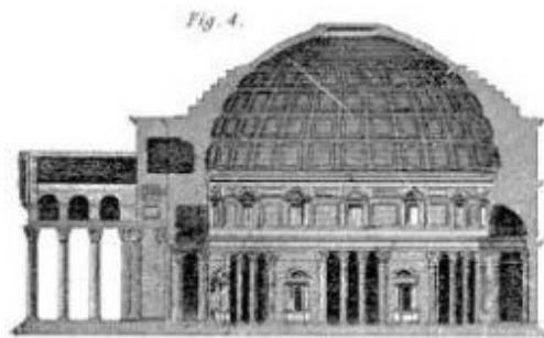
Section of Pantheon.
