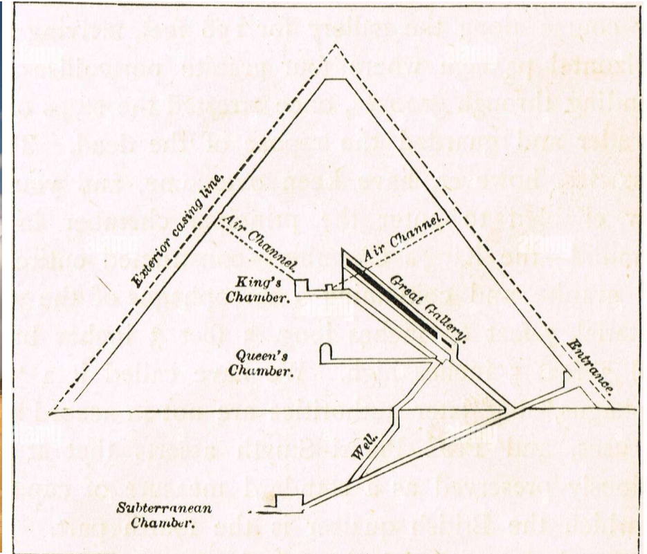
SECTION OF GREAT PYRAMID OF GHIZEH.
